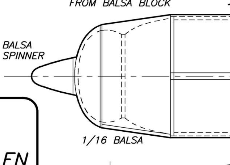
CARVE AND HOLLOW COWL FROM Balsa BLOCK
